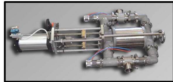
ABA-2000-PCV (power check valves)
